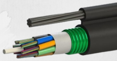
Overhead Antirodent Optical Fiber Cable (4 ~ 384C)
