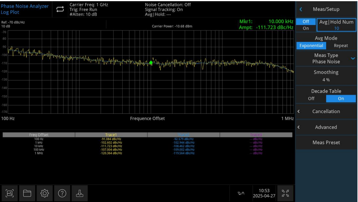
Phase Noise@10 kHz
