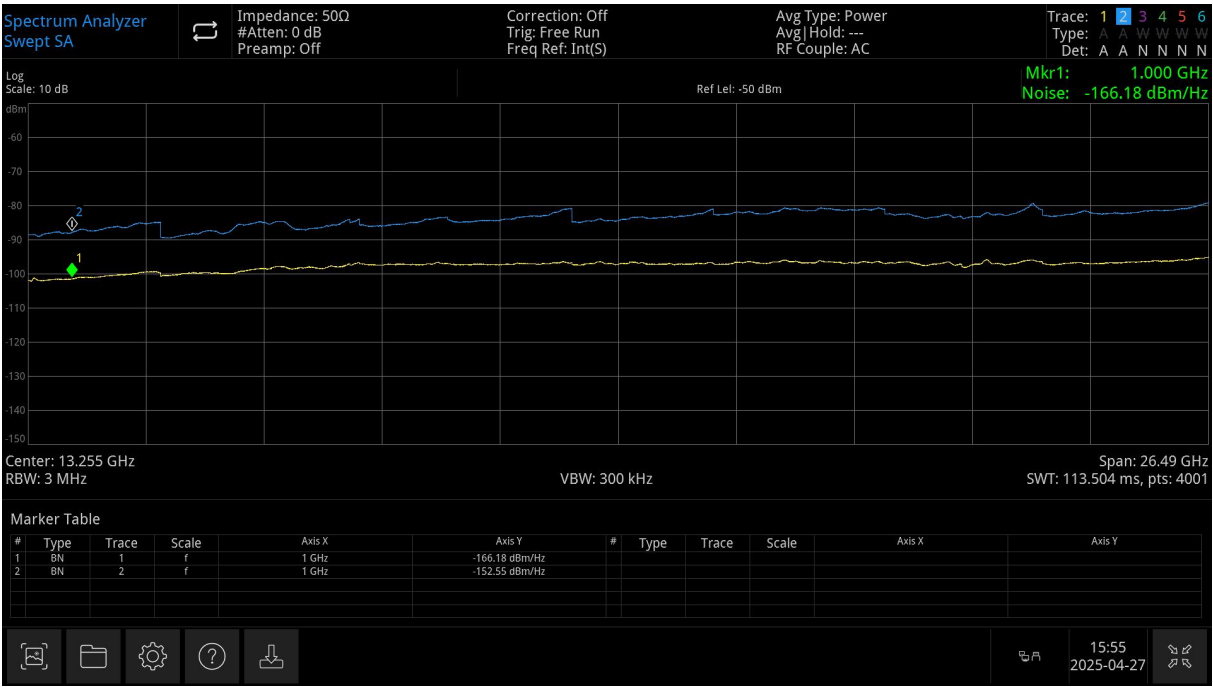
DANL (Preamplifier ON/OFF)
