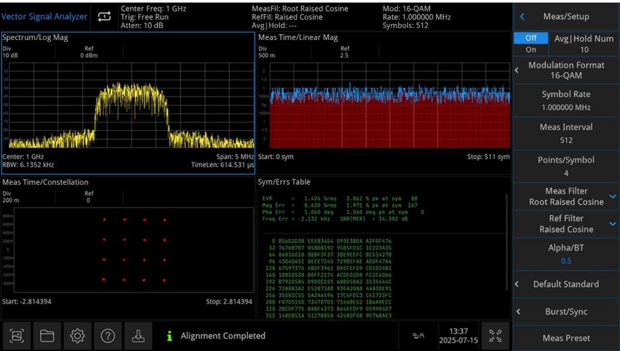
Vector Signal Analysis
