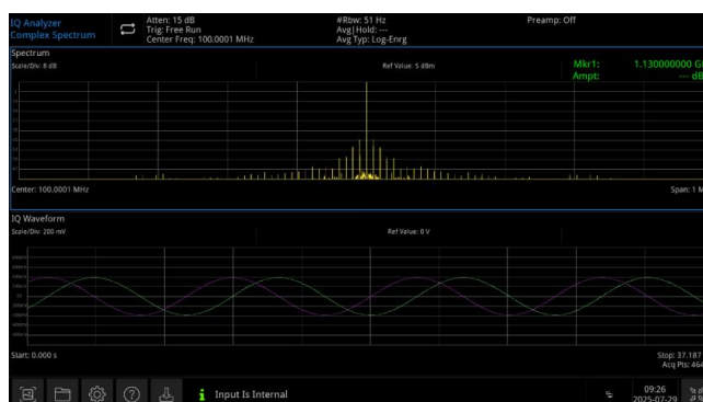
I/Q Analysis
