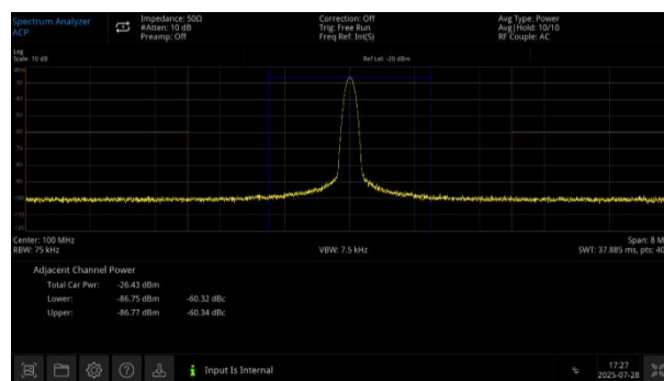
Enhanced Selectivity Adjacent Channel Power Measurement
