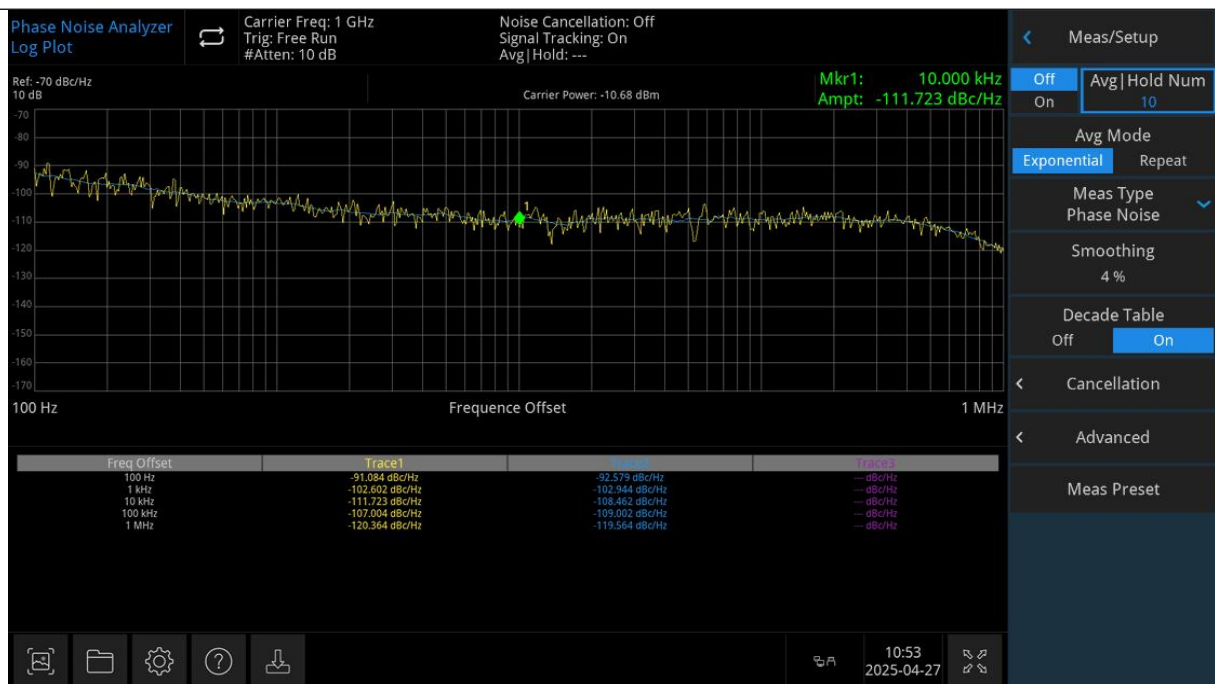
Phase Noise (Nom.) at 1 GHz Center Frequency
